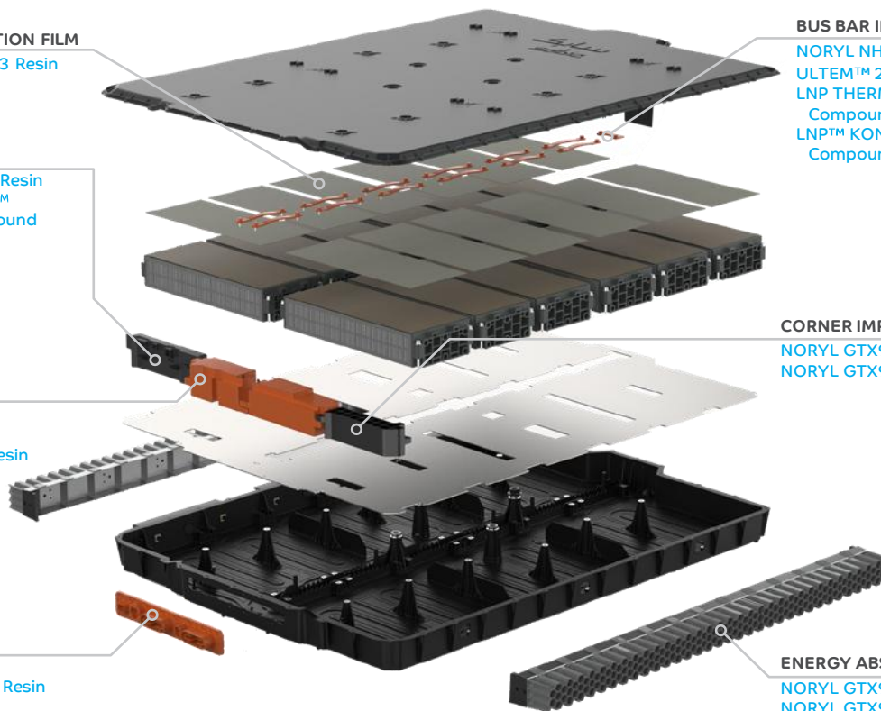
Exploded-view of battery pack showing diverse application potential for thermoplastics.
